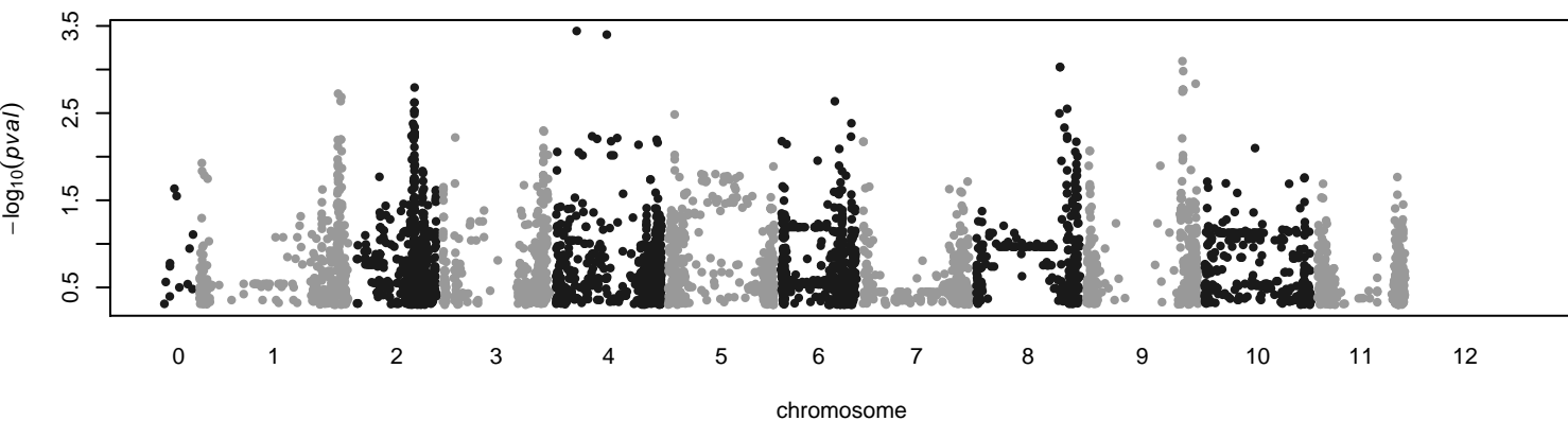
pval_ge
