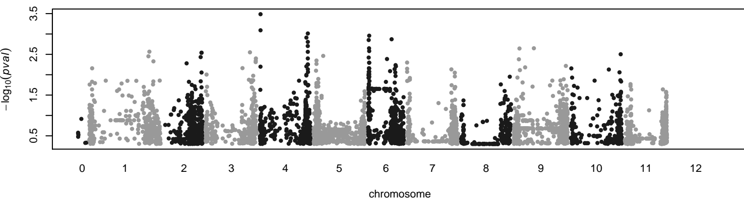
pval_full
